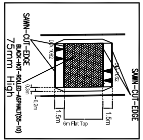
TYPICAL SPEED TABLE LAYOUT
